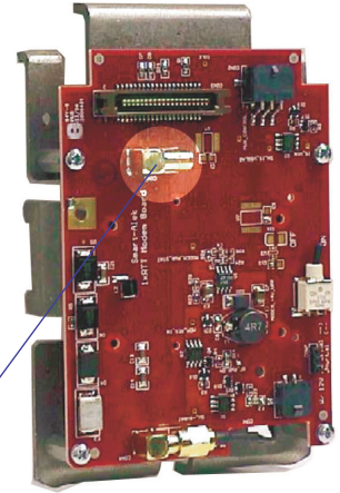
RF Cable Connection location
