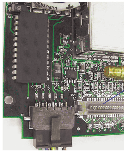
Figure 5 20x2 Signal Harness Connection on Modem Interface PCA
