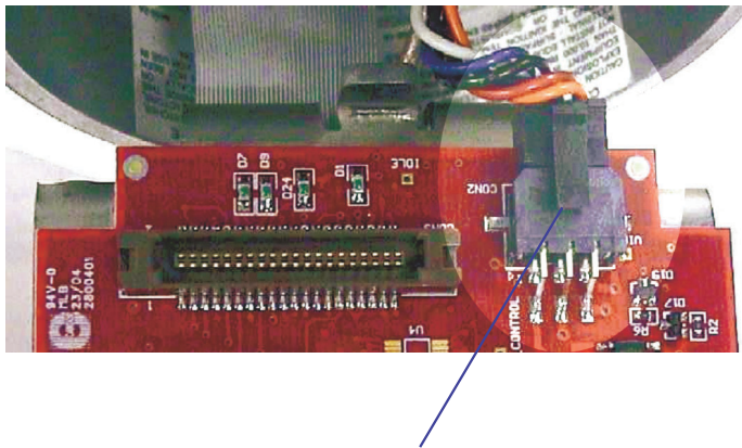
Figure 10 Power Harness Connection on Modem Interface PCA
