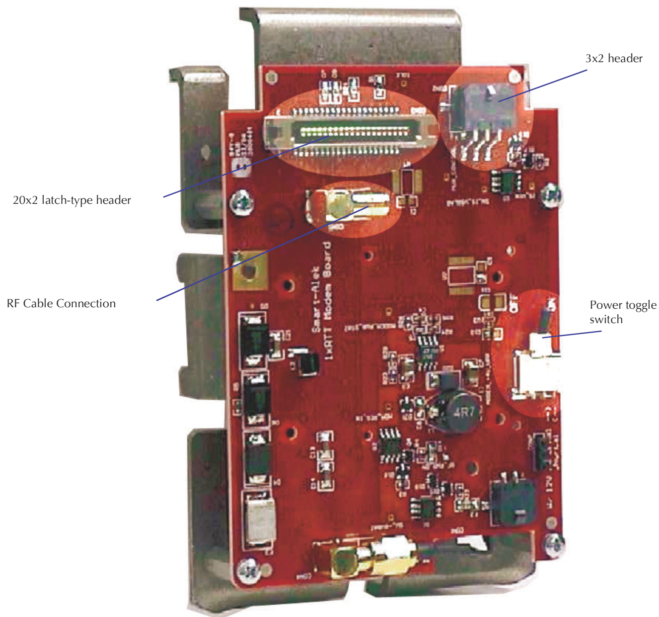
Figure 8 Typical Strongback-1XRTT Modem Unit
