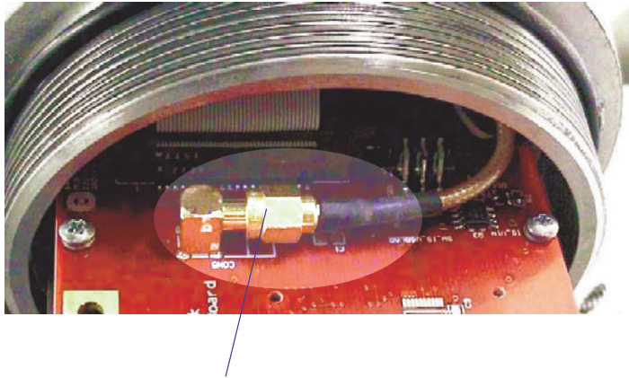
Figure 9 RF Cable Connection to Modem Interface PCA
