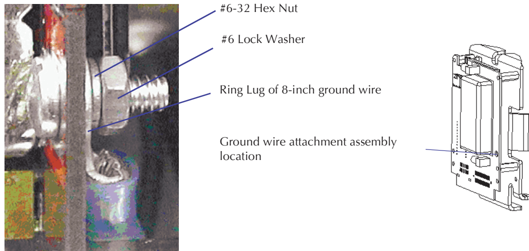
Figure 3 Ground wire attachment assembly Ground Wire Attached to Modem Interface PCA (Top of PCA on left side of photo, bottom side on right)
