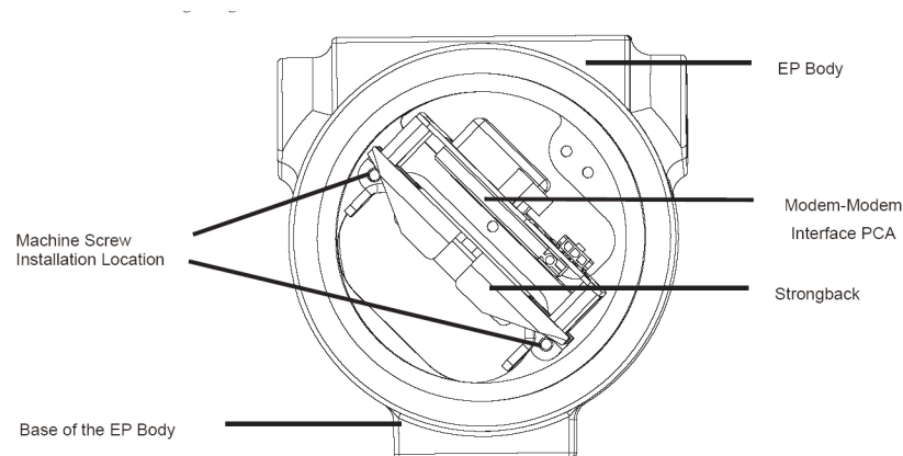
Figure 15 Strongback Installation into EP Body
