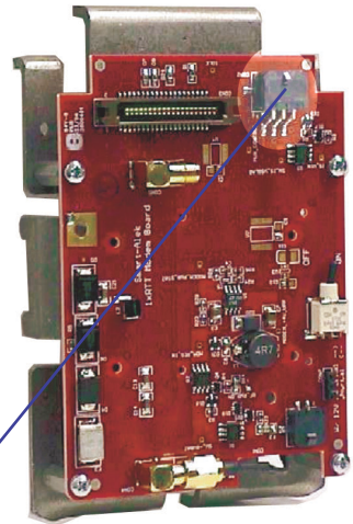
RF Cable Connection location
