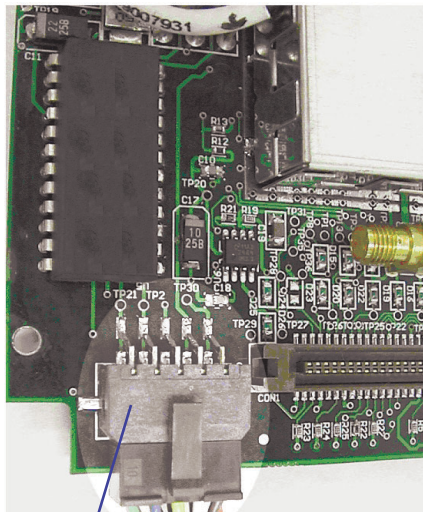
Figure 6 Power Harness Connection on Modem Interface PCA
