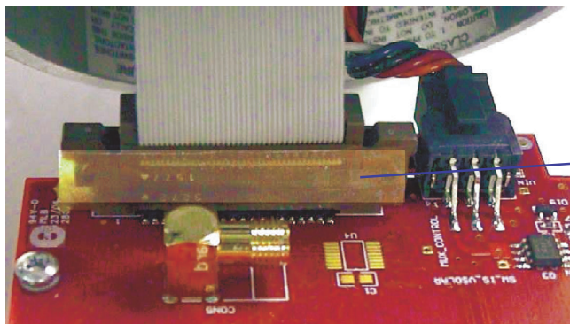
Figure 12 Kapton Tape Applied to the RF/Power Cable Side of the Signal Harness Connection
