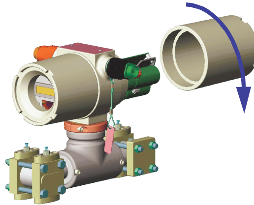
Figure 1 Removing the Back Dome Cover from the Explosion-Proof (EP) body. The Back Dome cover is threaded on. Turn left to remove.
